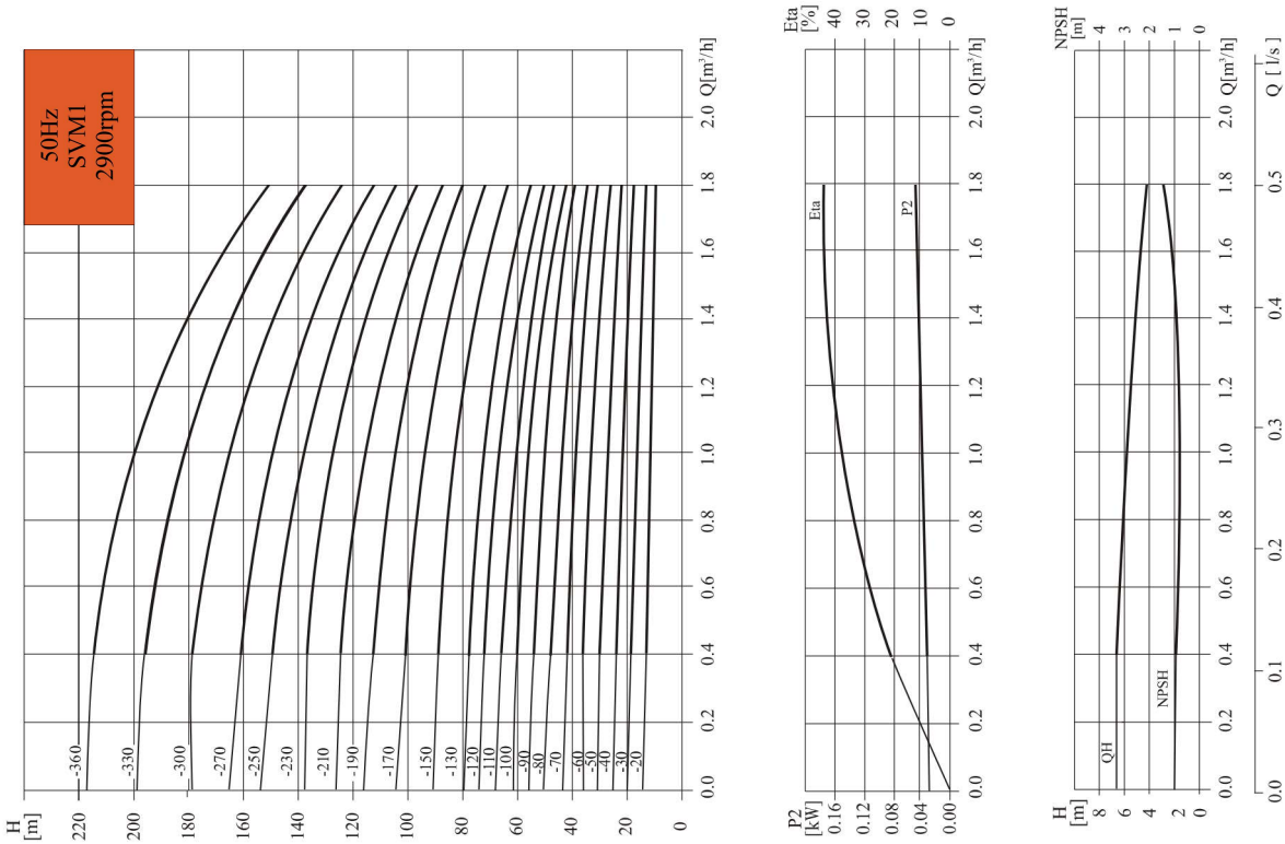
Performance curves
