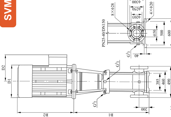
Installation drawing
