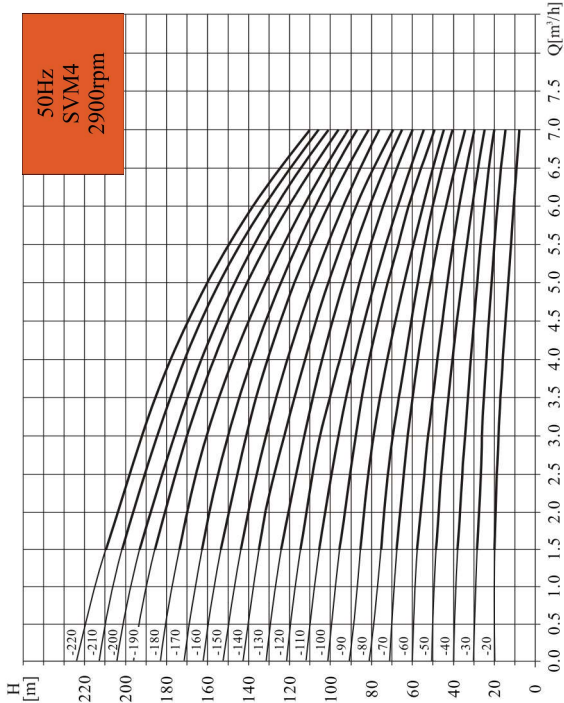
Performance curves
