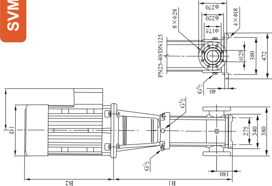
Installation drawing
