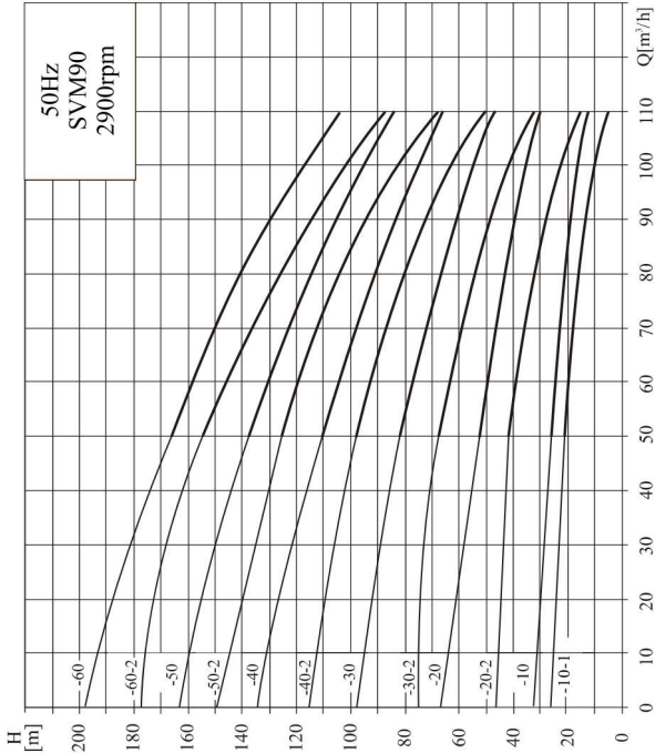
Performance curves
